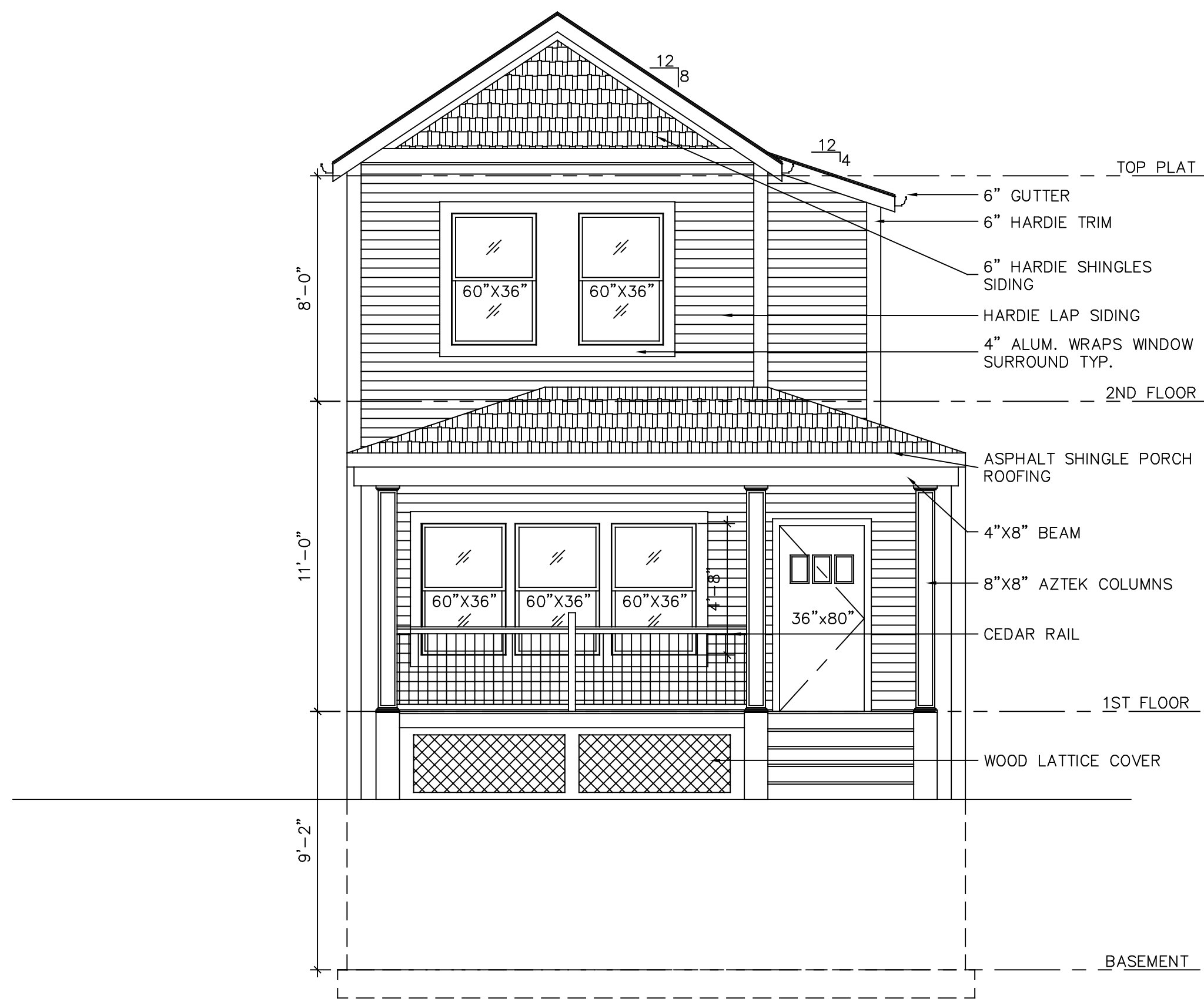
SOUTH ELEVATION 1/4"=1'-0"
