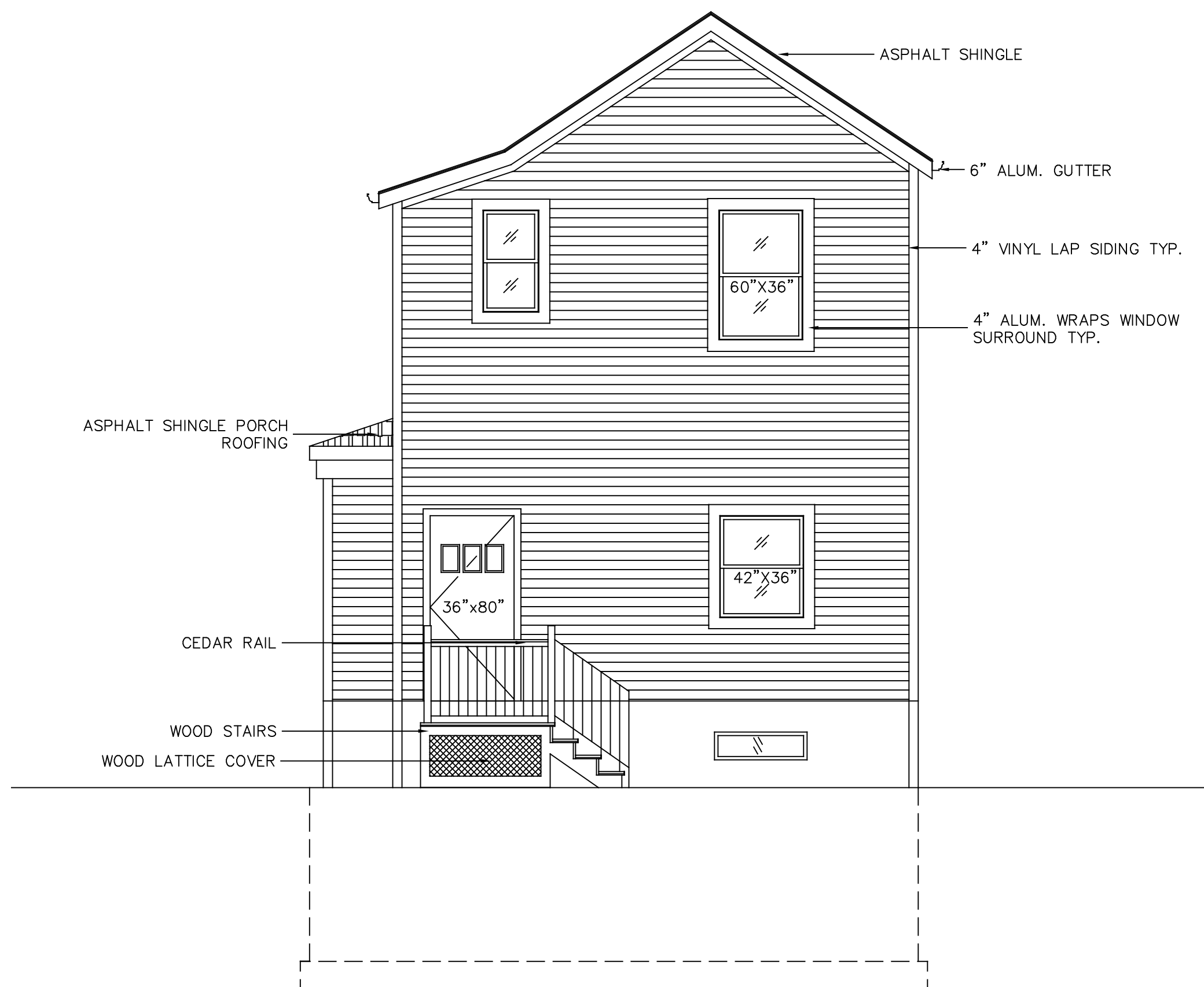
NORTH ELEVATION 1/4"=1'-0"
