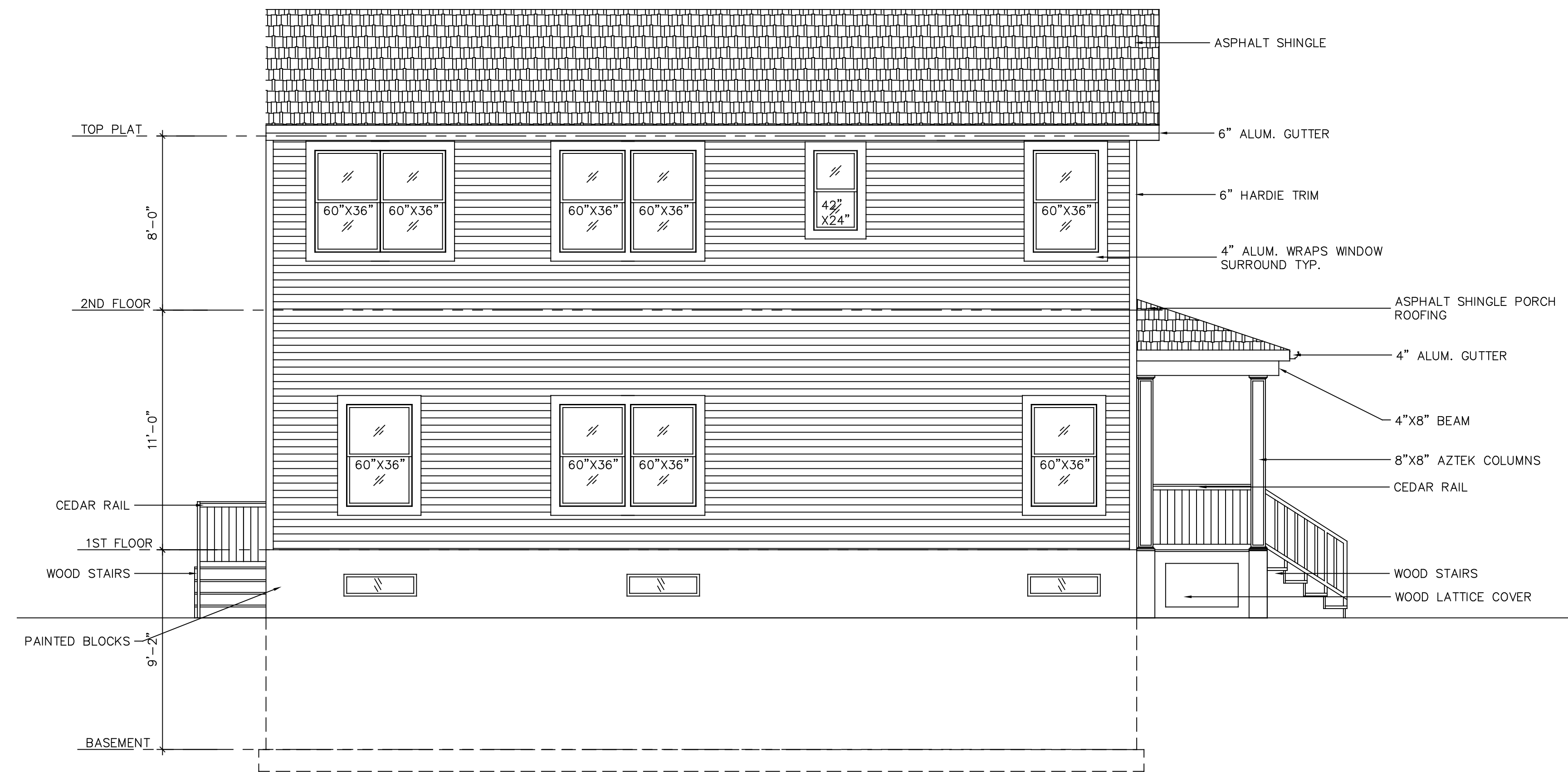
WEST ELEVATION 1/4"=1'-0"
